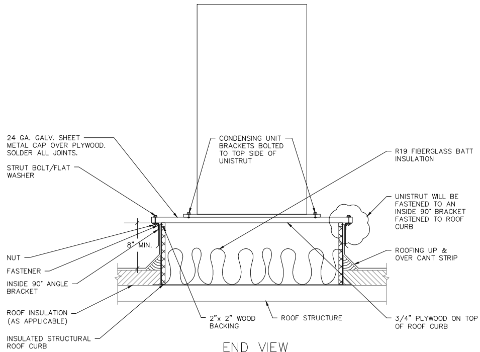
END VIEW
